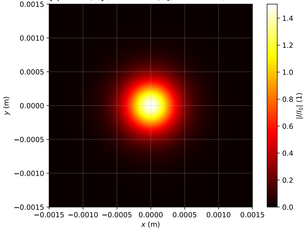
Intensity profile I(x, y, z = 3.423m)/I_0 , Pin=0.9Pcr, artificial time
